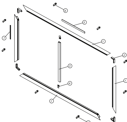
STANDARD LIP FRAME FRAME - Fixed Lite
