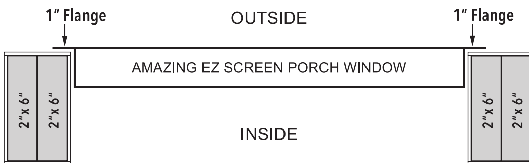
Standard Installation Top View
