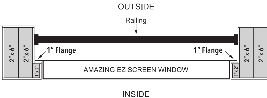
Recessed Installation Top View
