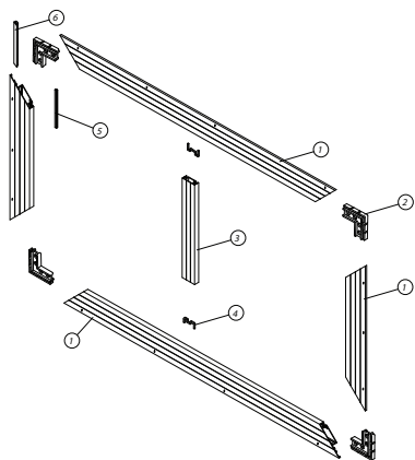
HEAVY DUTY LIP FRAME FRAME - Fixed Lite
